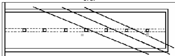
III. 68: Schematic drawing of cellar morgue 1 of Crematory II. Lengthwise, the concrete center beam with 7 supporting pillars. Shown as crossing lines: Flow lines showing midpoint of the three objects found on the roof. 558 Shaded rectangle: Location of the openings shown in III. 64 and 65.
