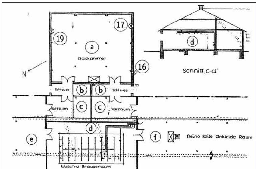
III. 77: Floor plan of HCN disinfection wing of Building in Auschwitz-Birkenau, and of Building 5a (mirror symmetrical) before its conversion. 601
