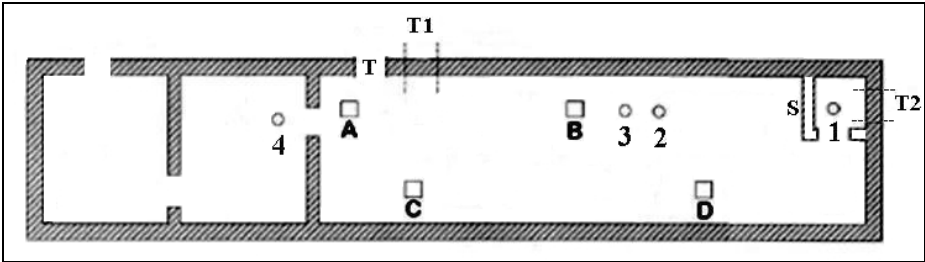
Document 15: Drawing of the morgue of crematorium I with rooms to the left (original state). A,B,C,D: position of current openings in the roof. 1, 2, 3, 4: position of original circular openings, today closed. T: original door to the furnace room; T1: current opening to the furnace room; T2: Current access door from the outside; S: Current vestibule, included when converted into an air raid shelter. © Carlo Mattogno
