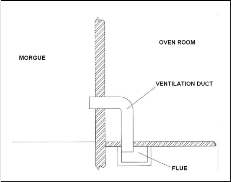
Document 11: Schematic diagram of first, makeshift ventilation installation for morgue of crematorium I at Auschwitz. Vertical section. © Carlo Mattogno
