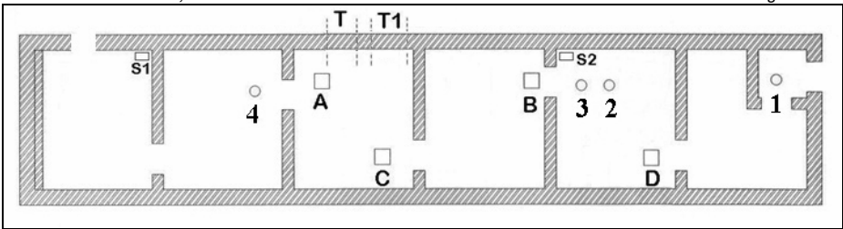
Document 16: Drawing of the morgue with rooms to the left after conversion to air raid shelter. A,B,C,D: position of current openings in the roof. 1, 2, 3, 4: position of original circular openings, today closed. T: original door to the furnace room. T1: current door (both were closed during the use of this facility as an air raid shelter). S1, S2: position of air raid shelter's ventilation shafts. © Carlo Mattogno
