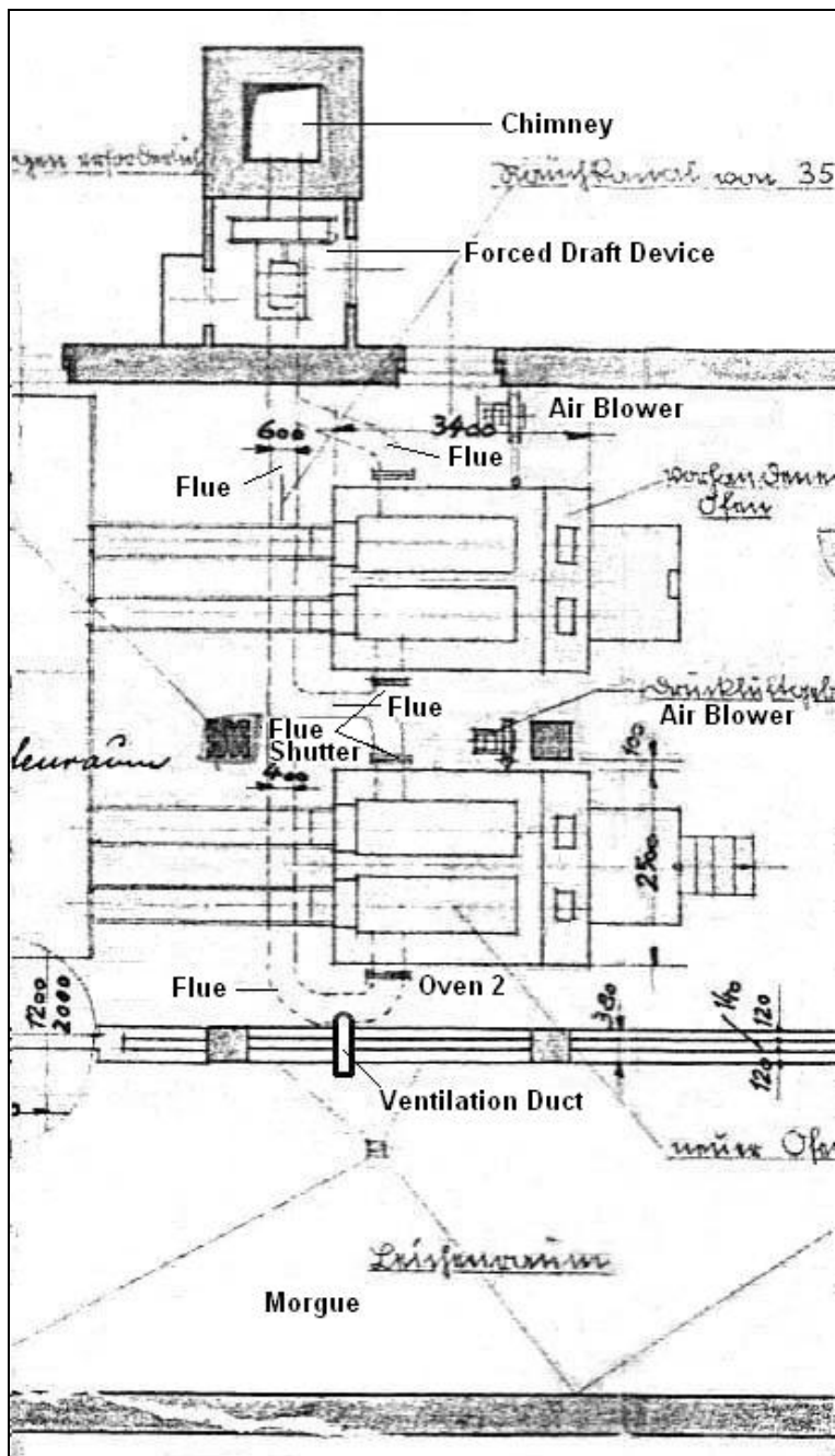
Document 10: Schematic diagram of first, makeshift ventilation installation for morgue of crematorium I at Auschwitz. Horizontal section of Topf drawing D 57999, dated November 30, 1940.
